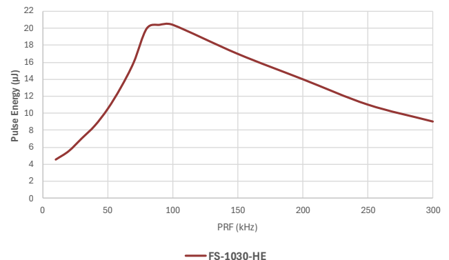
Pulse Energy Vs. PRF
