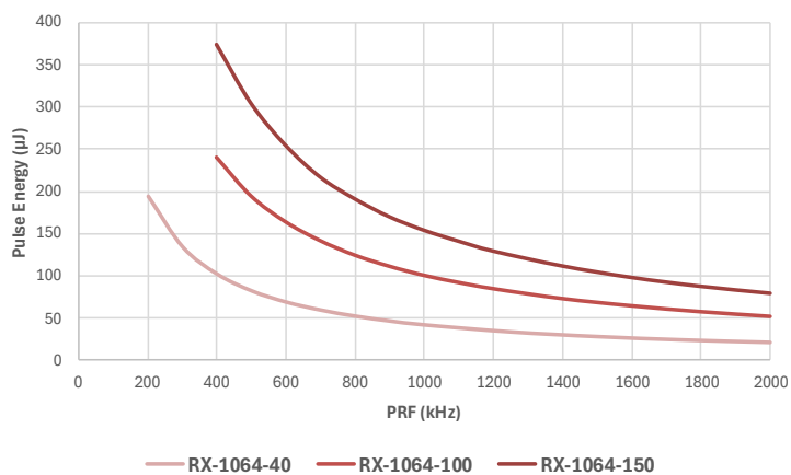
Pulse Energy Vs. PRF
