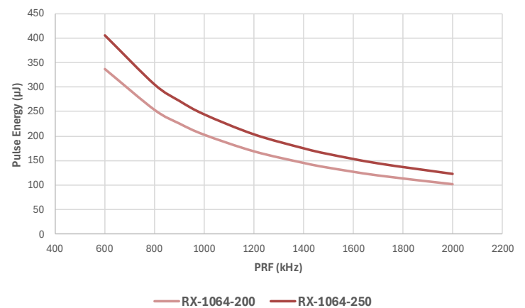
Pulse Energy Vs. PRF
